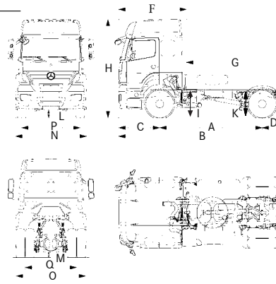
Axor 1840 LS/4x2/3600
