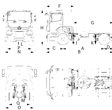
Axor 1836 LS/4x2/3600
